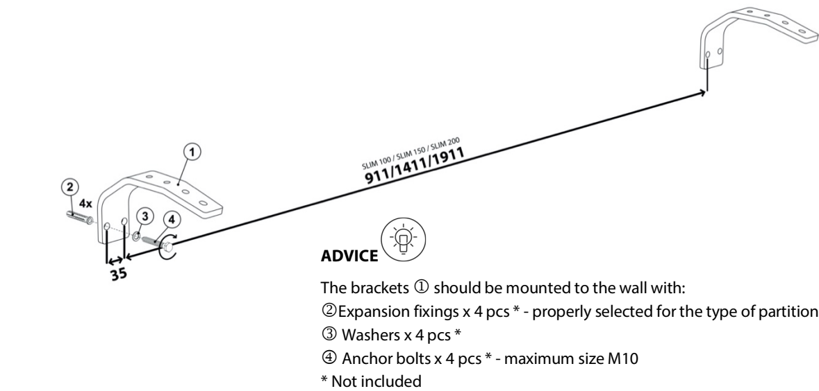
PIC 10.1. MOUNTING BRACKETS SPCING.
