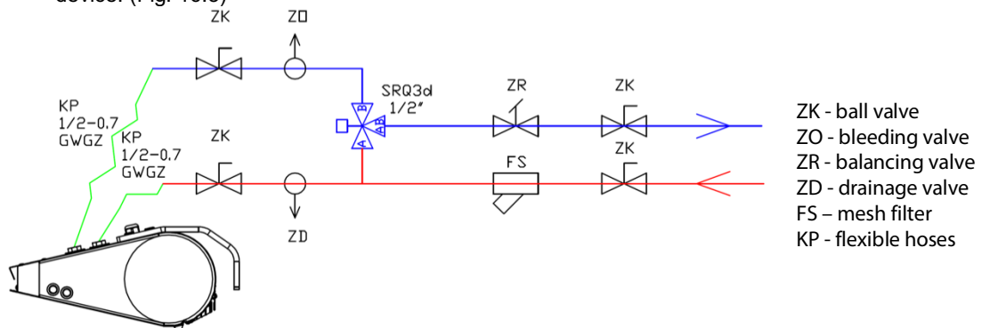
PIC. 17.3 CONNECTION EXAMPLE OF HYDRAULIC COMPONENTS.
