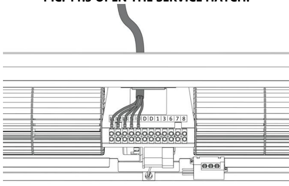
PIC. 11.3 OPEN THE SERVICE HATCH.
