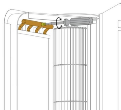
PIC. 17.2 BLEEDING/ AIR RELEASE VALVE.
