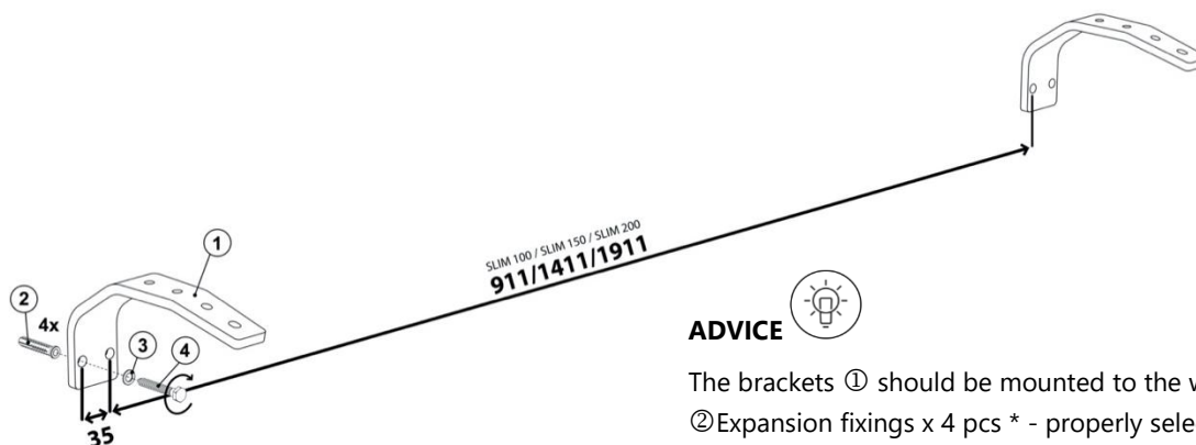
PIC 10.1. MOUNTING BRACKETS SPCING.
