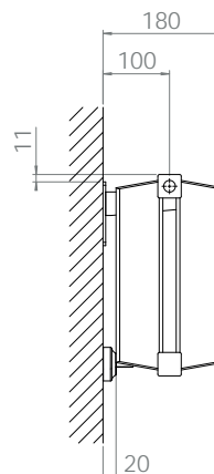
SC dobbelt (SCD) type 24 el. 26, profil
